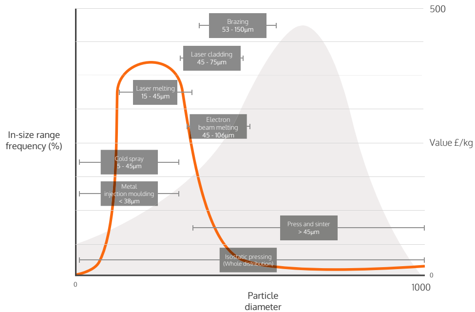
Atomisation Powder Size Distribution & Value
